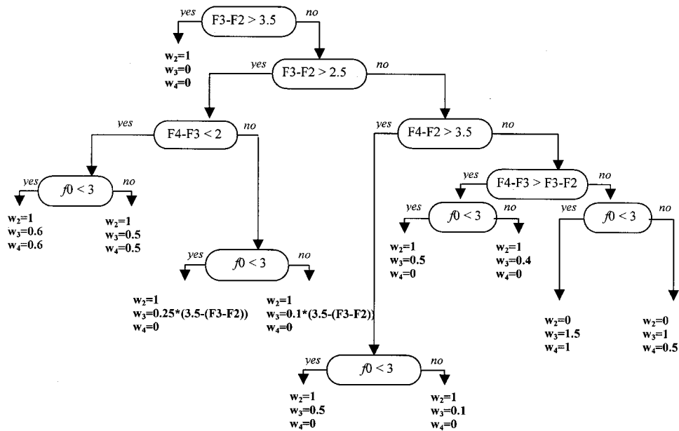
FIG. 3. F2' computation flow chart. F2' is defined by F2' = (w_2F2 + w_3F3 + w_4F4) / (w_2 + w_3 + w_4) (were w_2 \geq w_3 \geq w_4 , for w_i \neq 0 ). F2' is set at F2 , if F3 and F2 are two widely spaced; the contribution of F4 is included if F2 and F3 are close; if F2 , F3 , and F4 are within 3.5 Bark, F2' is set at the center of gravity of F2 and F3 or F3 and F4 , depending on the pattern of distances between the three formats; for high f_0 values, the weight of F3 and F4 is reduced. All values in Barks.
