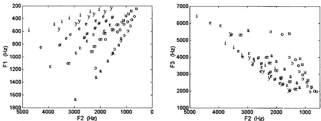
FIG. 2. Representation of the stimuli in the F1/F2 and F2/F3 spaces.
