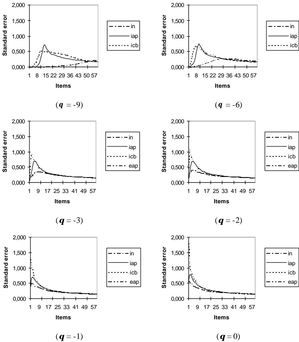
Figure 2. Standard error of the proficiency estimate according to the number of items administered
